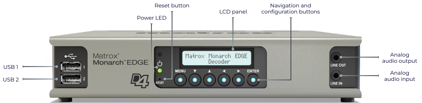
Matrox Monarch EDGE D4 (front view)
